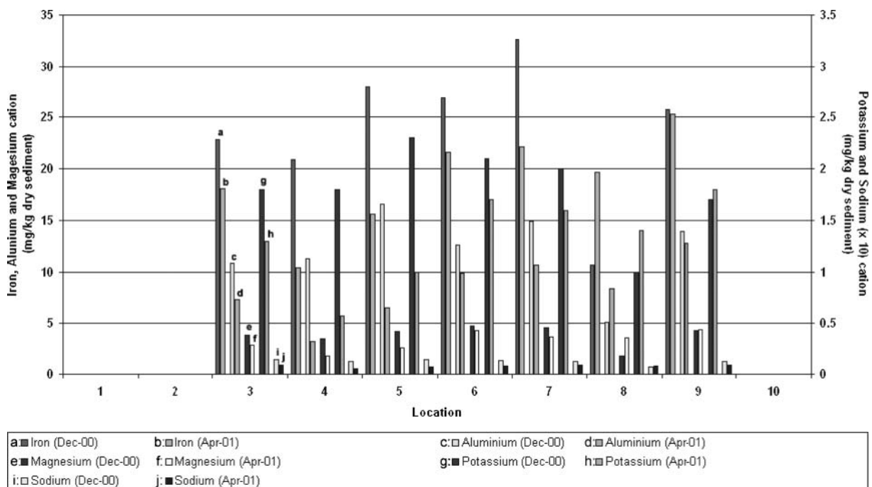
Fig. 4. Histograms of the concentrations of the major cations in sediments (mg/kg).
