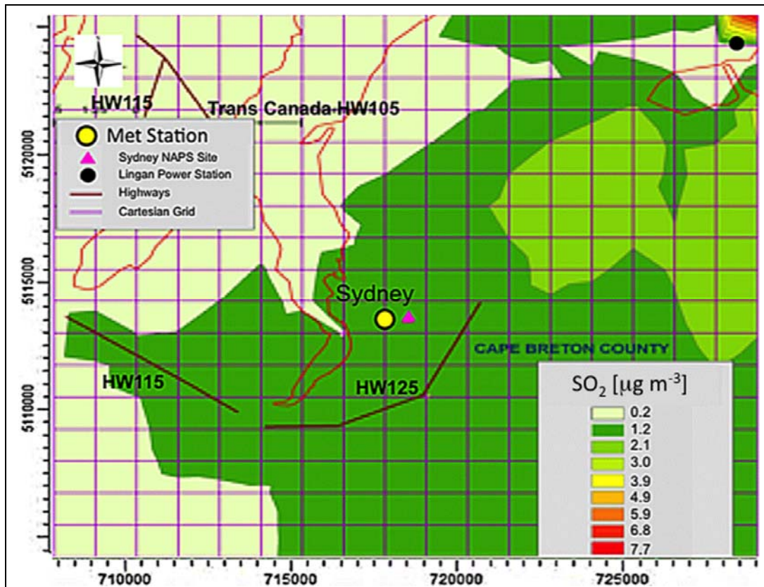
Figure 6. AERMOD estimated surface concentration of SO 2 SYD domain.
