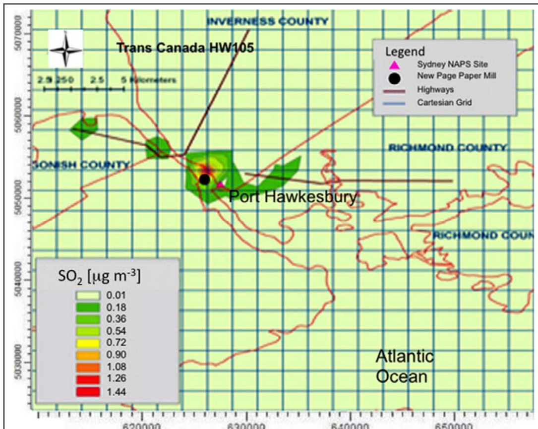
Figure 7. AERMOD estimated surface concentration of SO 2 PRTHWKS domain.
